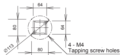
Detailed view Z
